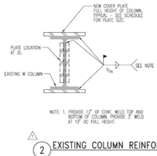
Figure 1: Existing Column Reinforcing Detail
