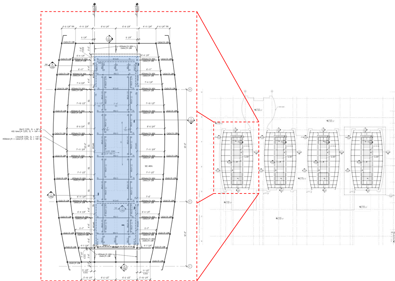
Figure 4: Lantern Framing Plan
