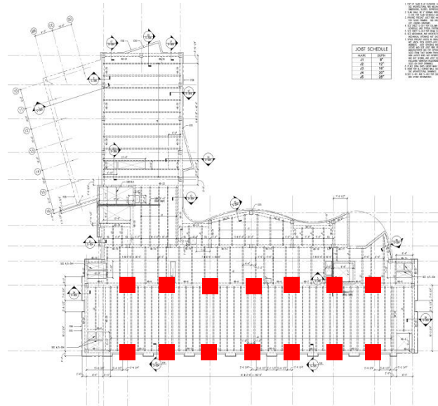
Figure 6- Floor plan showing the 6,000 psi column in basement and 1 floor
