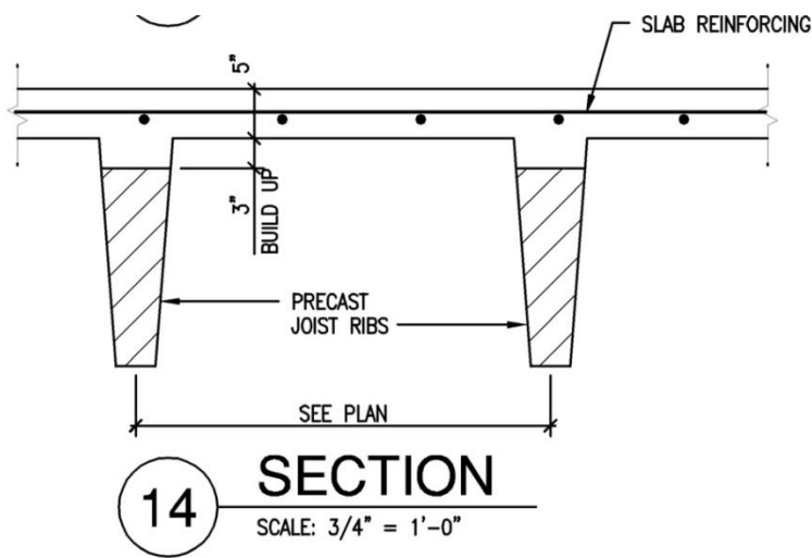
Figure 5- Plan and section of precast joists
