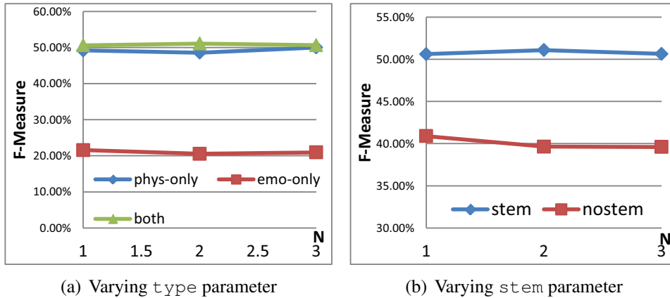
Figure 4: Parameter comparison of ST feature extraction as the function of maximum gram size (N).
