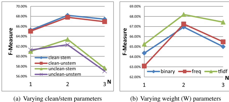
Figure 1: Parameter comparison of NG feature extraction as the maximum size of grams ( N ).
