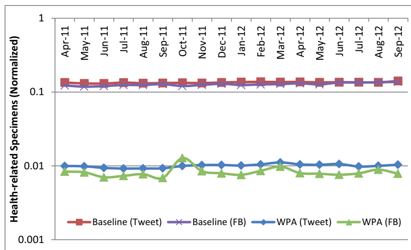
Figure 5: A complete run of our best method (WPA) against the baseline on both the TwitterB and Facebook datasets captured during the period of 18 months from April 2011 to September 2012.
