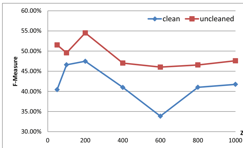
Figure 3: Parameter comparison of TD feature extraction as the function of number of topics (Z).
