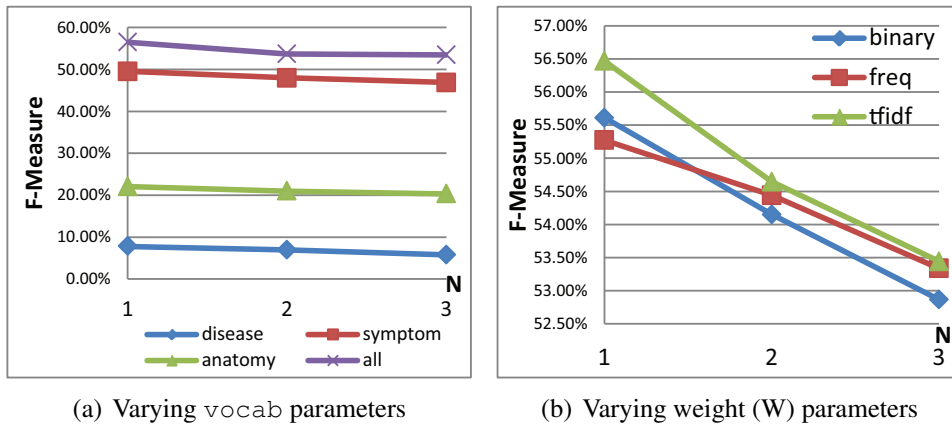
Figure 2: Parameter comparison of DC feature extraction as the function of maximum gram size (N).
